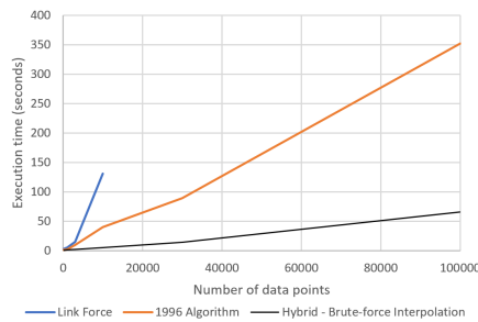
(a) Execution time for up to 100,000 data points of Poker Hands data set (b) Relative stress of each finished layout compared to Link Force of different data sets
