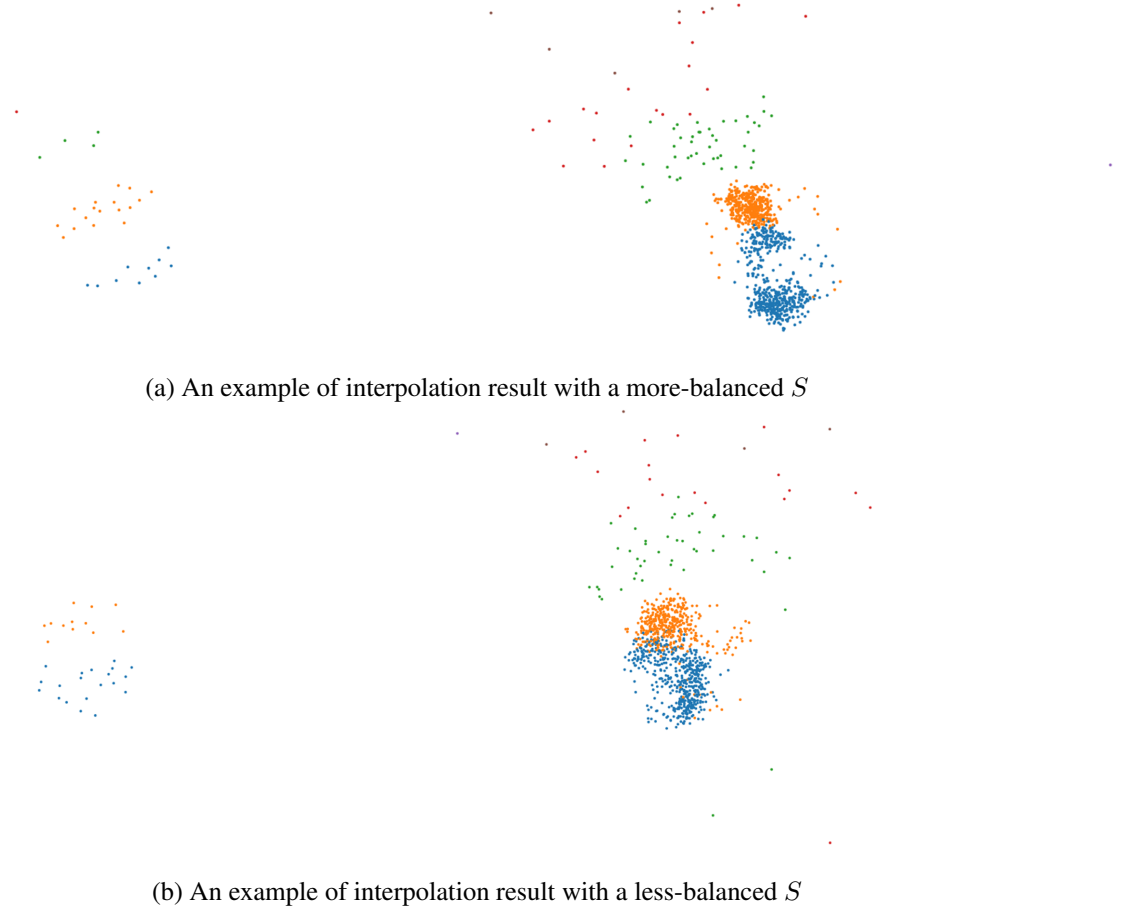
Figure 5.4: Difference in interpolation results of a subset with 1,000 data points. Left images show only data points in set S and the right show the interpolation result.
