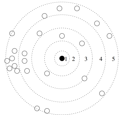
Figure 2.3: Diagram of a pivot (dark shaded point) with five buckets, illustrated as discs between dotted circle. Each of the other points in S are classified into buckets by the distances to the pivot.
